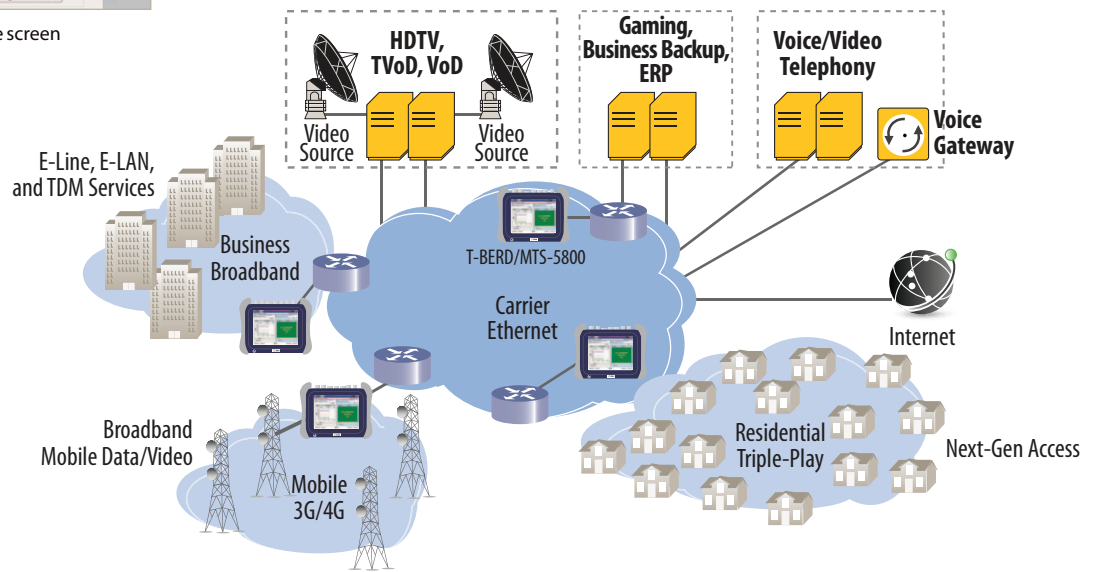
Carrier Ethernet Network
