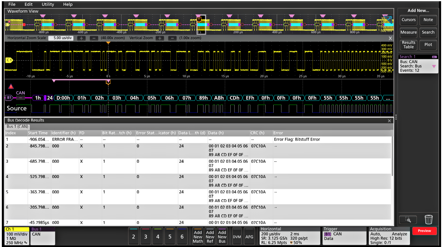
Triggering on a CAN serial bus. A bus waveform provides time-correlated decoded packet content including Start, Arbitration, Control, Data, CRC and ACK while the bus decode table presents all packet content from the entire acquisition.
