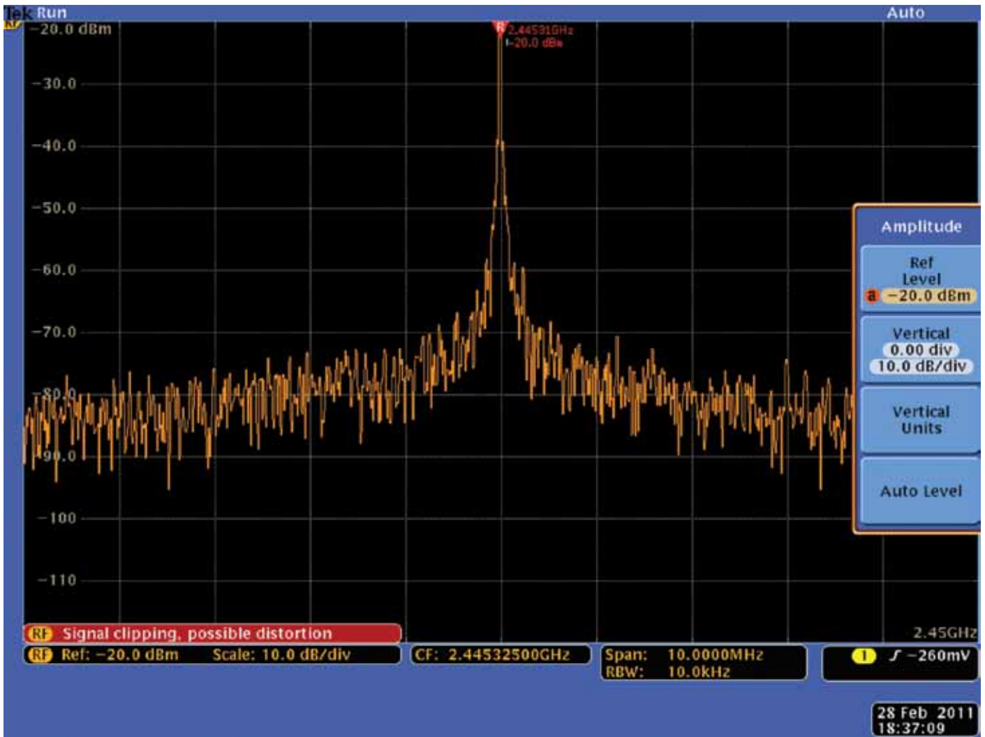
Figure 24. Clipping Indicator.
