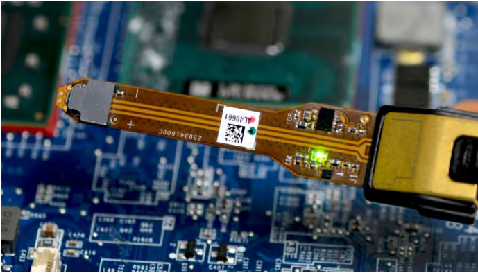
P77STFLXA solder down, flex circuit accessory with an active buffer amplifier on its tip provides up to 20 GHz bandwidth.
