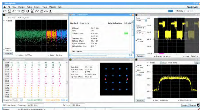
DPO770002SX with SV30 provides industry best EVM accuracy, it allows easy setup to perform transmitter measurements including time overview of the bursts, spectrum, constellation diagram, decoded burst information and EVM measurements.
