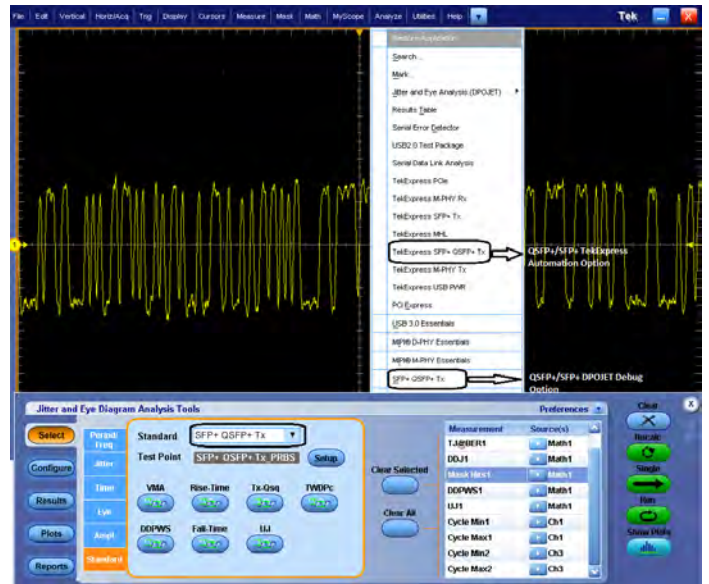
Tektronix SFP+ QSFP+ Tx - is developed on a Real Time Oscilloscope platform, which is the platform of choice for engineers designing their products around SFF-8431 & SFF-8634 technology. Option SFP-TX and SFP-WDP enable both an Automation Solution (for Compliance) and DPOJET Option (for Debug). Users can save up to 80% on testing time compared to manual testing. TWDPc - Transmitter Waveform Distortion Penalty for Copper Measurements are available with Option SFP-WDP. SFF-8431 SFP+ TWDPc based Matlab code is integrated into the SFP-WDP option to make sure Engineers can use this measurement in the automated setup.
