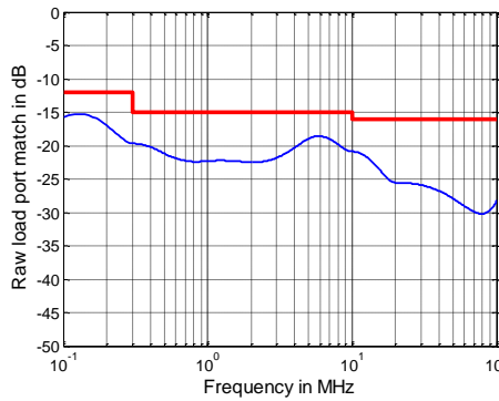
Raw load port match versus frequency for the R&S ® ZNBT20
