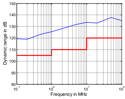
Dynamic range in dB versus frequency for the R&S®ZNBT26/R&S®ZNBT40
