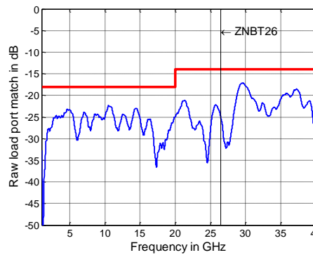
Raw load port match versus frequency for the R&S ® ZNBT26/R&S ® ZNBT40
