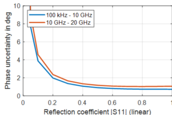
Uncertainty of reflection magnitude and reflection phase measurements for the R&S®ZNB20 in the frequency range from 100 kHz to 20 GHz; analysis conditions: S_{12} = S_{21} = 0 , cal. power -10 dBm, meas. power -10 dBm
