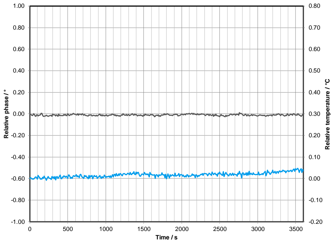
Measured relative phase between two LO coupled R&S®SMW RF paths vs. time, carrier frequency = 2 GHz, level = -10 dBm (the lower curve / right vertical axis indicates the temperature variation)
