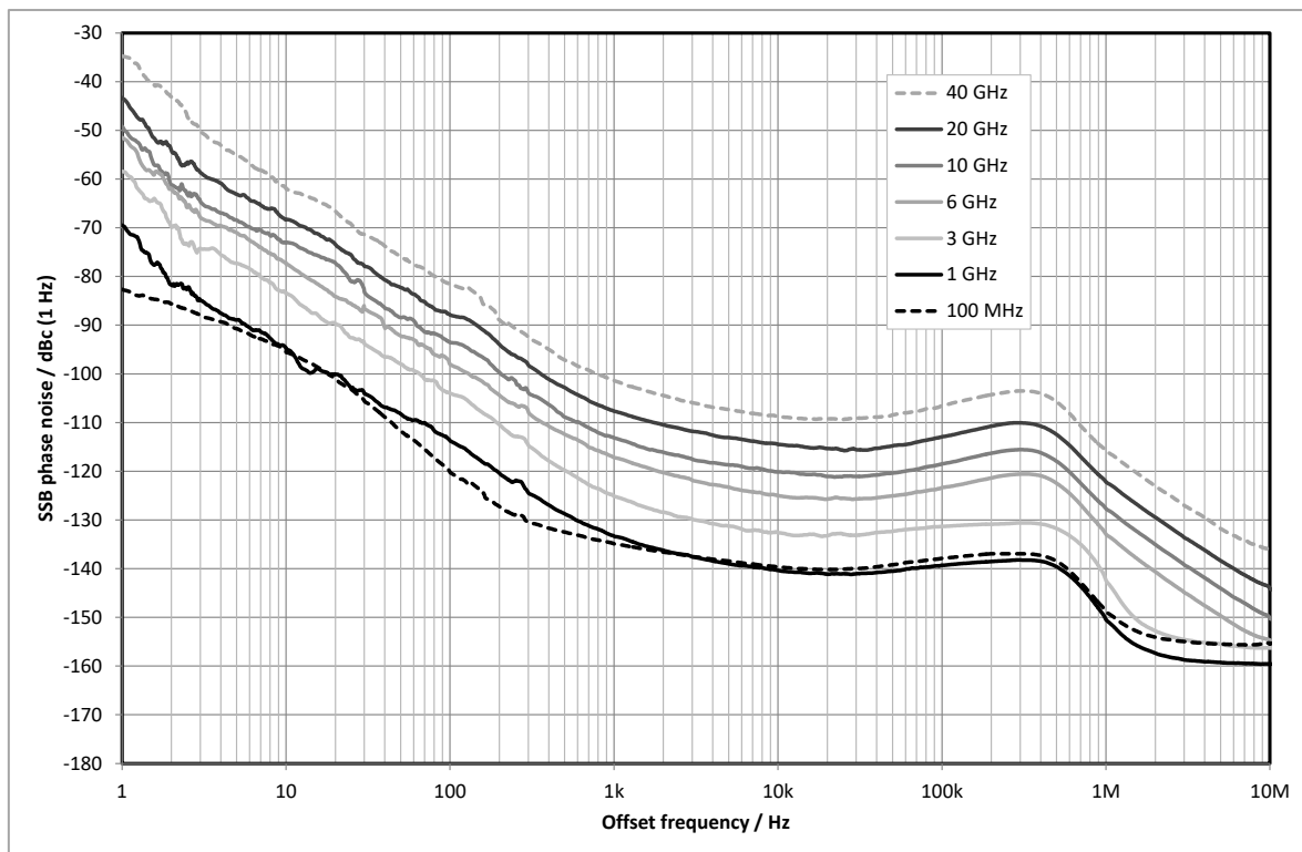
Measured SSB phase noise performance with R&S®SMW-B22 option, CW mode
