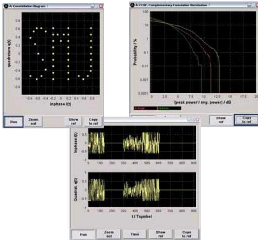
Graphics block with constellation, CCDF and I/Q diagrams
