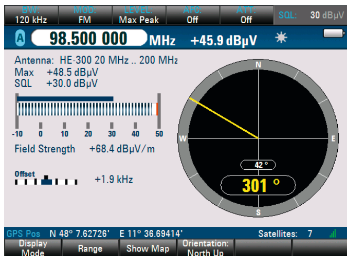
Direction finding of a signal source with the R&S®HE400 active directional antenna.
