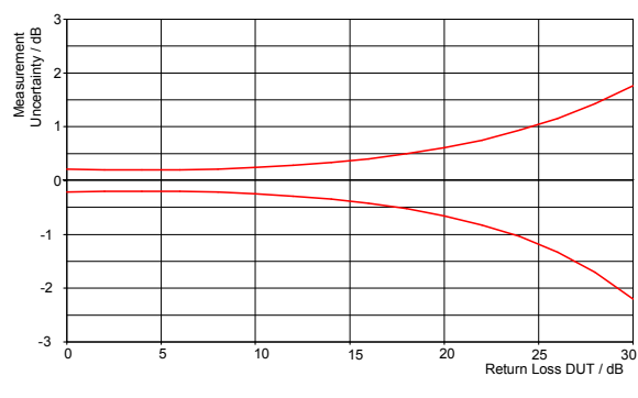
Measurement uncertainty with vector measurements (option R&S FSH-K2)
