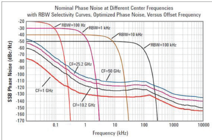
Keysight MXA Signal Analyzer Screen Display
