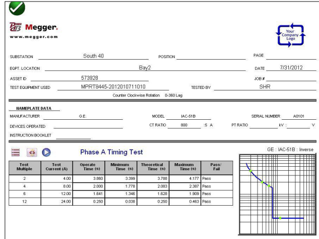
Figure 5: Test report G.E. IAC-51B inverse timing test
