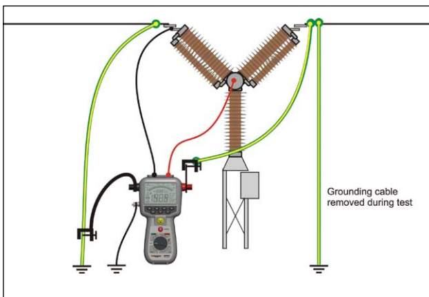
Traditional measurement from ground. Injection is done through existing grounding cable (earthing). Optional cable kit is needed. Available kits have 5, 10 or 15 m cables.
