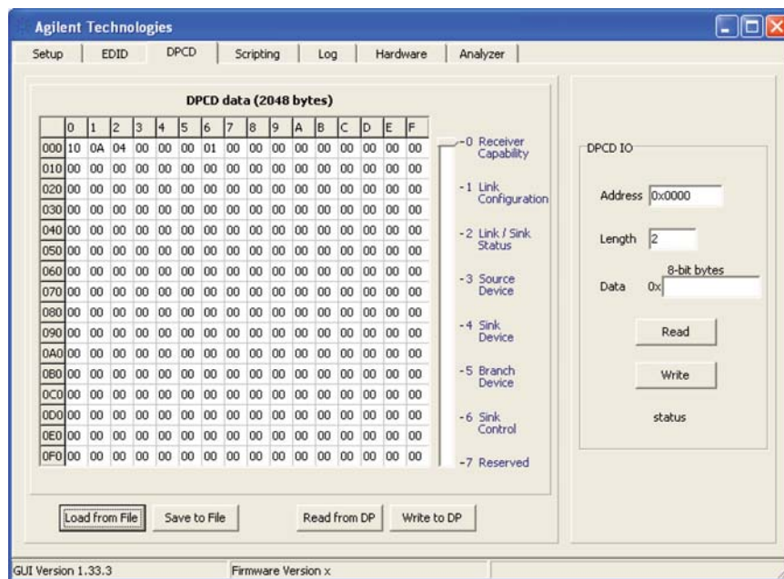
Figure 4: DPCD tab screen for the W2642A GUI
