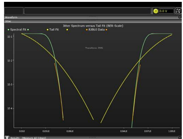
Determine which algorithm fits your data best
