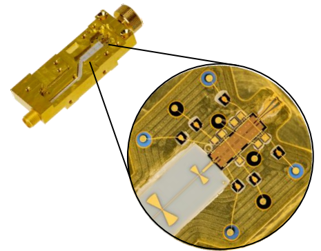
An Indium Phosphide enabled high-speed step generator lies at the heart of every Infiniium calibration module
