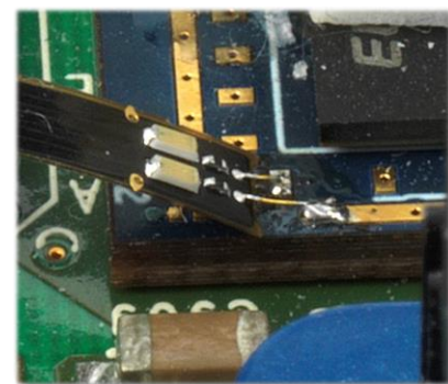
MX0100A InfiniiMax II Micro Probe Head
