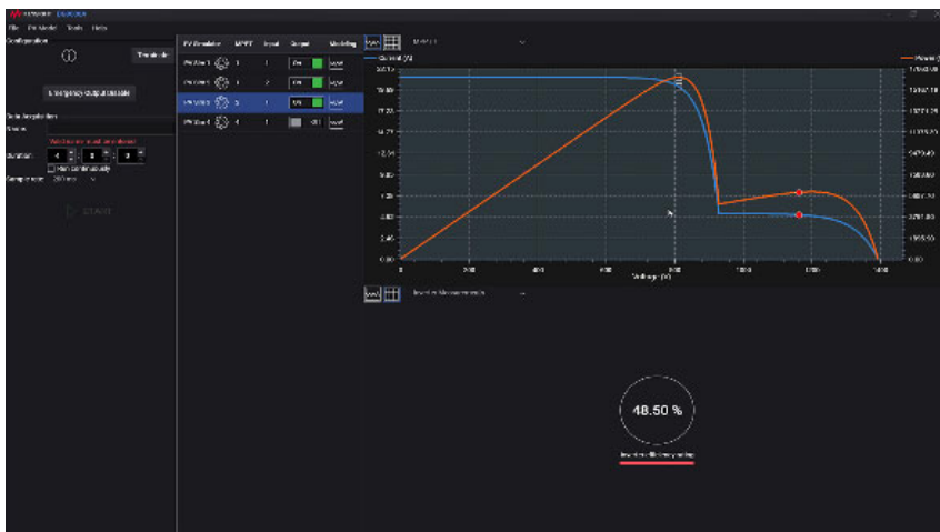
Figure 4. DG9000A MPPT efficiency
