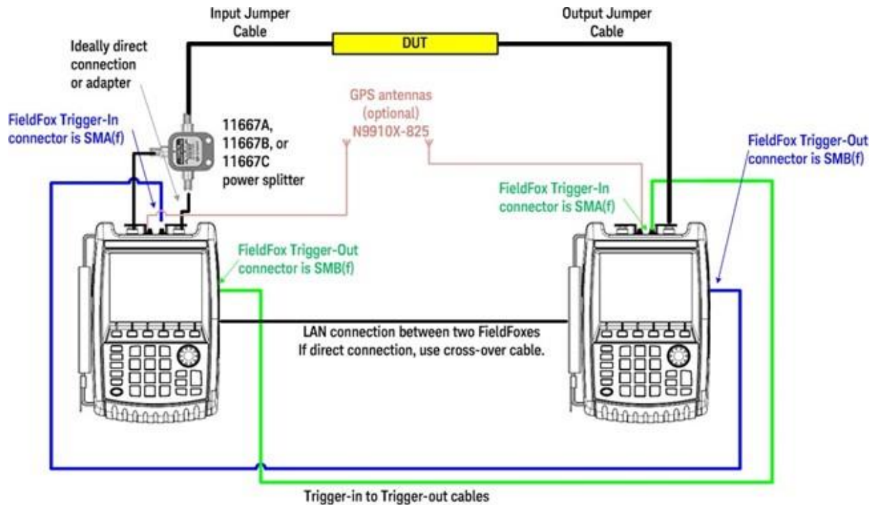
Figure 1. ERTA system diagram
