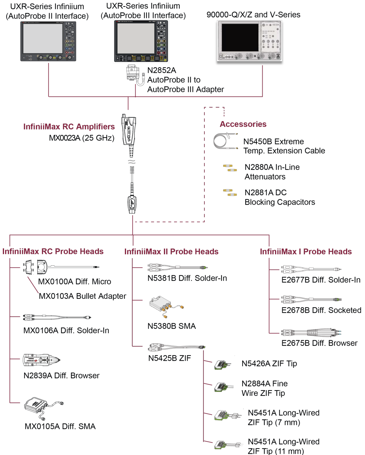
InfiniiMax RC probing system family diagram
