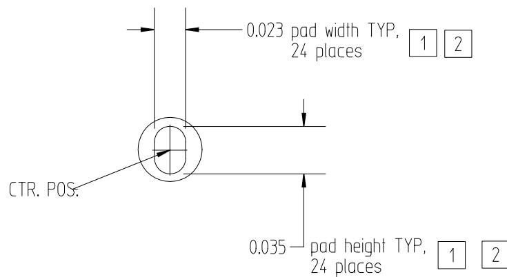
Figure 44 Dimensions of N5328A
