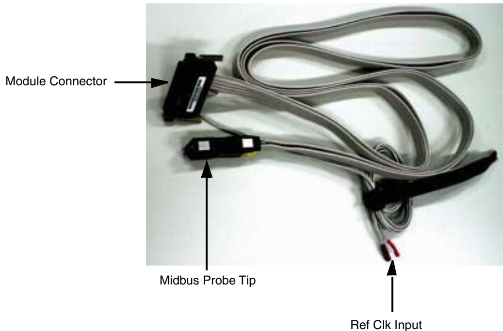
Figure 42 N5328A Half Size Midbus Probe
