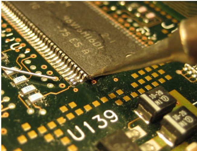
Figure 65 Solder Added to Target Points
