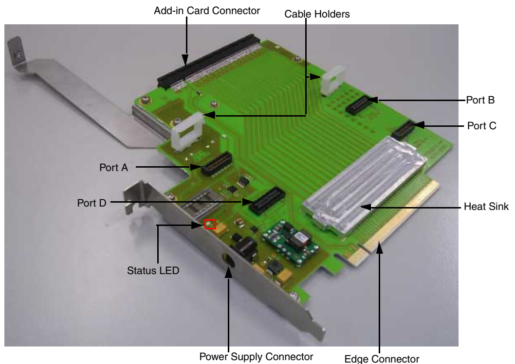
Figure 15 N5315 Solid Slot Interposer Card
