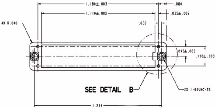
Figure 29 Dimensions of the Retention Module and its Parts
