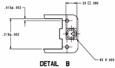
Figure 30 Dimensions of the Retention Module and its Parts
