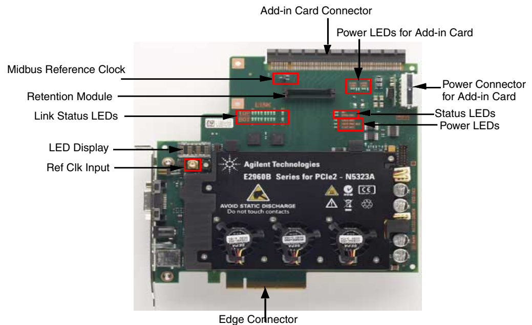
Figure 11 N5323A Jammer Card
