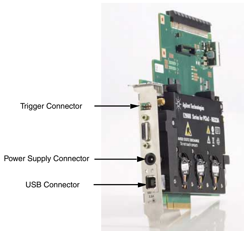
Figure 14 N5323A Jammer Card
