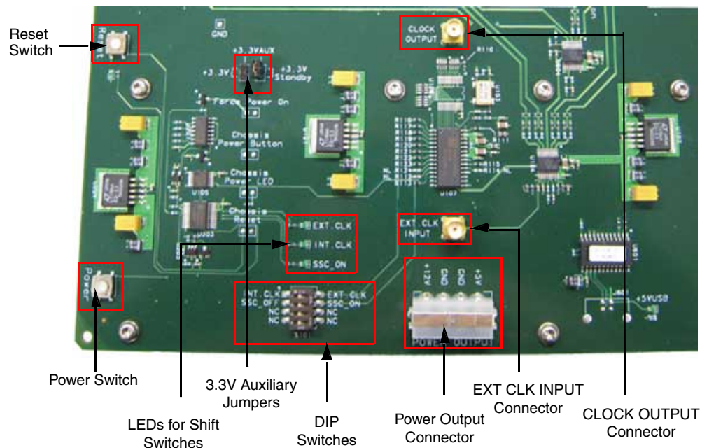
Figure 20 N5316A Backplane Board Components
