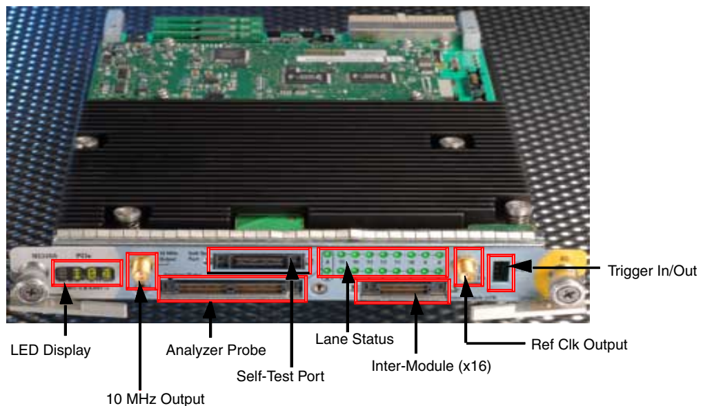
Figure 1 N5306A I/O Module
