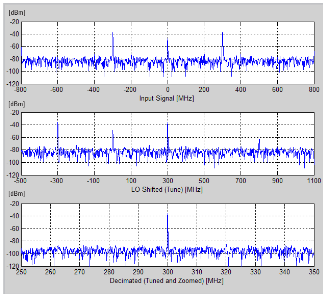
Figure 6. Example of the DDC functionality. The 1st graph shows the FFT of a 300 MHz sinusoid signal being digitized at 1.6 GS/s, then the LO is set to shift the center frequency at the signal frequency and finally a decimation ratio of 16 is applied, reducing the analyzed bandwidth to 100 MHz around the signal of interest.
