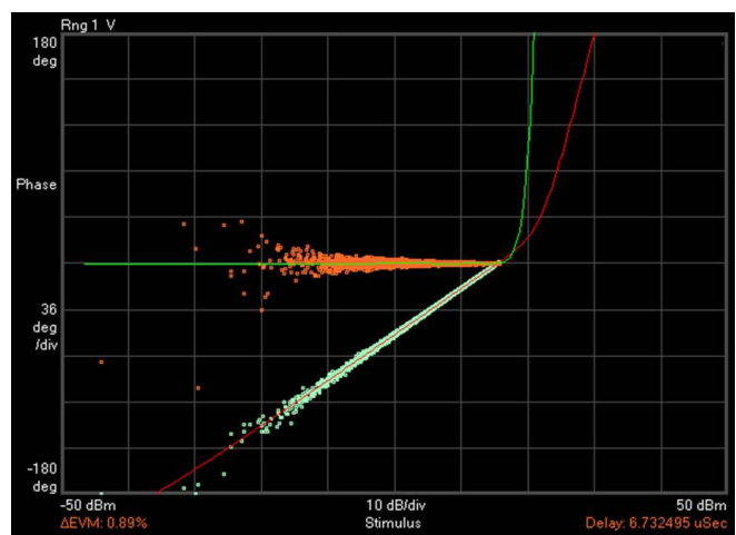
Figure 17. AM/AM and AM/PM characteristic for a 16QAM 250 MSym/s LTE signal at 400 MHz IF frequency and 400 MHz analyzed bandwidth.
