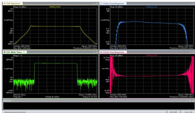
Figure 7. The excellent channel-channel phase coherency, coupled with the wideband and flexible capability of the -DDC option, allows exceptionally fast and accurate cross-channel measurements on a large variety of signals, such as multi-tone, wideband frequency chirps, or complex signals. In this case, we show the measurement of cross-channel phase and amplitude for a 160 MHz frequency chirp.
