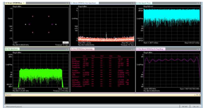
Figure 9. The M9703A wideband digital receiver allows to directly digitize DVB-T signals with excellent dynamic range without the need of analog mixers, especially interesting for passive radar applications.
