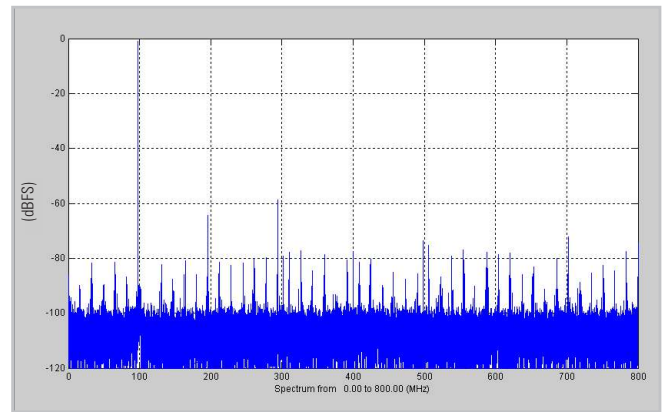
Figure 12. The FFT plot for a -1 dBFS input signal at 100 MHz in 1 V FSR shows the excellent dynamic range of the M9703A high-speed digitizer.
