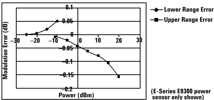
Figure 2-3 Wideband CDMA Error of Agilent E-Series E9300 power sensor versus corrected CW sensor
