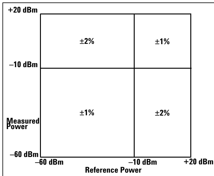
Figure 3-5 Relative Mode Power Measurement Linearity with Agilent EPM power meter at 25 °C ±10 °C (typical)
