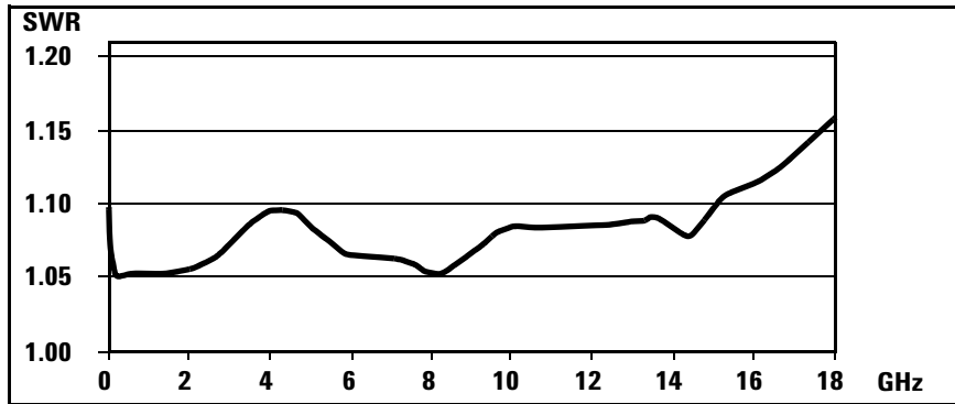
Figure 3-1 Typical SWR 10 MHz to 18 GHz (25 °C ± 10 °C)
