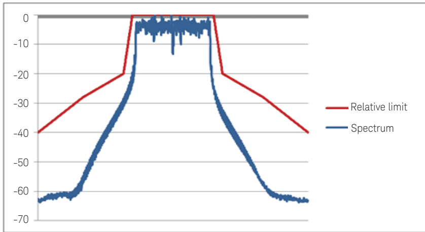
Figure 3. 802.11a/g SEM nominal performance at 5.8 GHz with 20 MHz bandwidth
