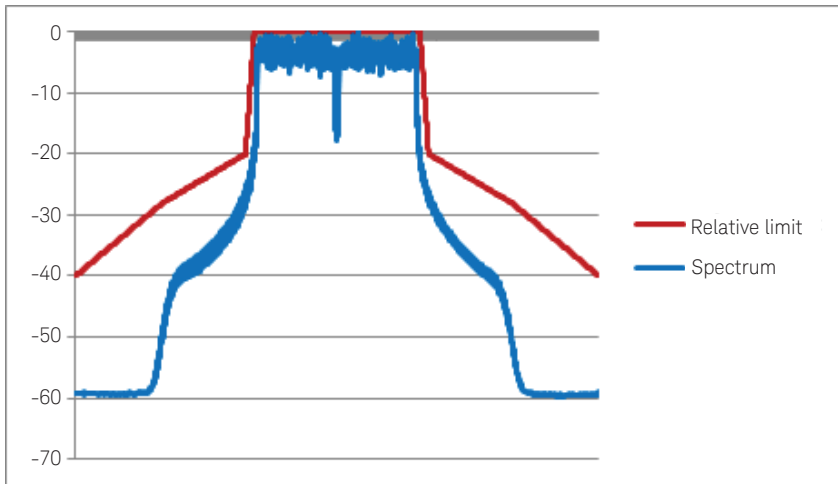
Figure 4. 802.11n SEM nominal performance at 5.8 GHz with 40 MHz bandwidth
