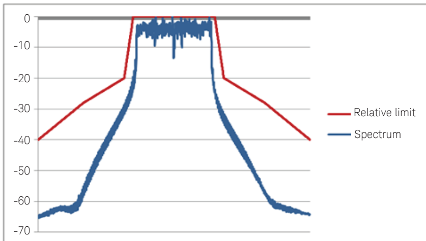
Figure 2. 802.11a/g SEM nominal performance at 2.4 GHz with 20 MHz bandwidth
