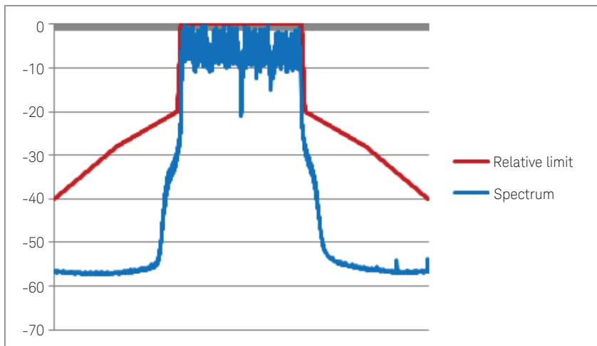
Figure 5. 802.11ac SEM nominal performance at 5.8 GHz with 80 MHz bandwidth
