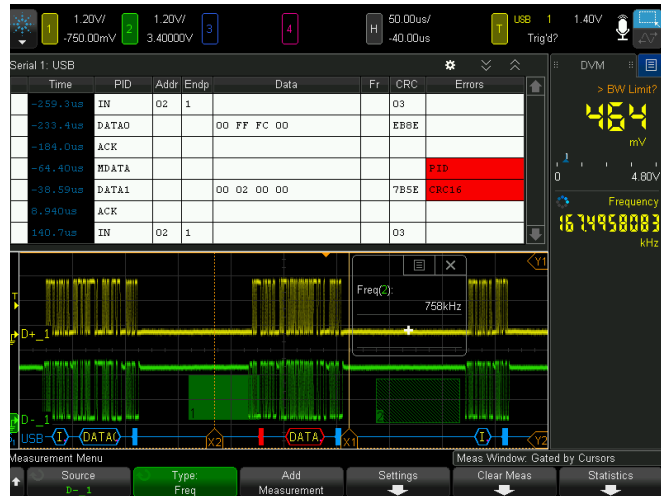
Figure 30. USB 2.0 protocol trigger and decode option display.
