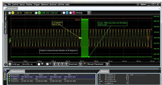
Figure 58. N8900A Infiniium Offline software.
