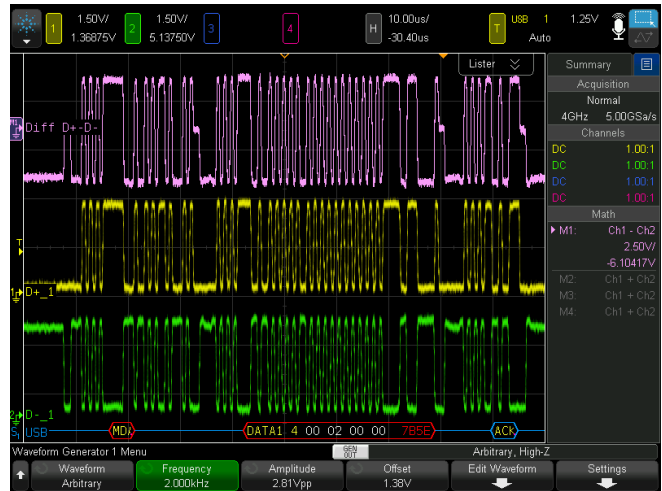
Figure 29. Dual-channel generator generating a differential signal.
