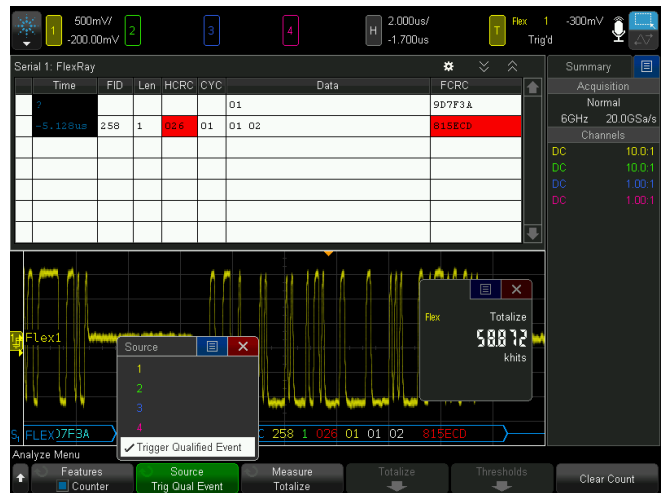
Figure 34. Totalizing the number of CAN errors.
