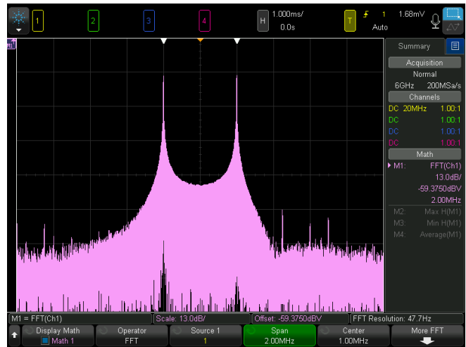
Figure 36. Traditional monochrome FFT with limited features.
