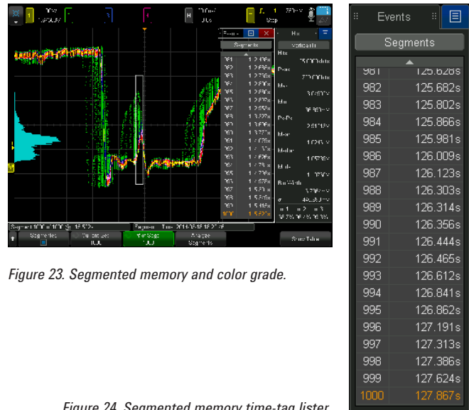
Figure 24. Segmented memory time-tag lister.
