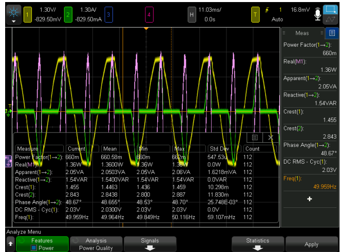
Figure 43. Power quality analysis screenshot.
