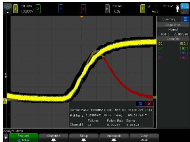
Figure 40. Limit testing of infrequent glitch.
