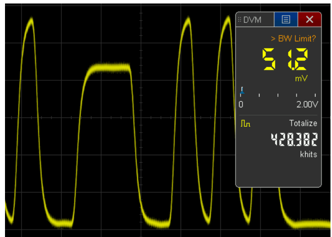
Figure 35. Totalizing the number of runt errors.
