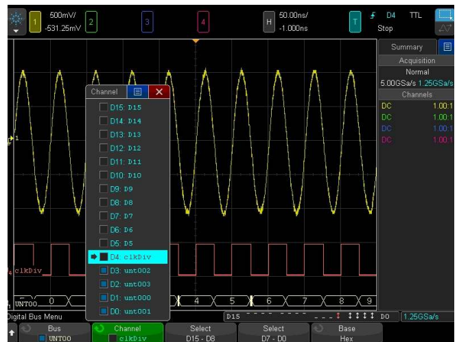
Figure 46. FPGA dynamic probe screen.
