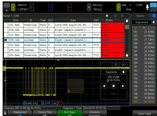
Figure 25. Segmented memory + serial bus decode + InfiniiScan Zone trigger.
