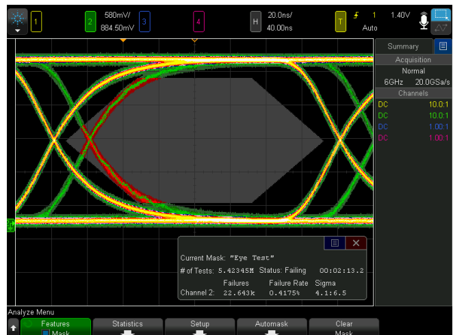
Figure 41. Mask testing of serial data.
