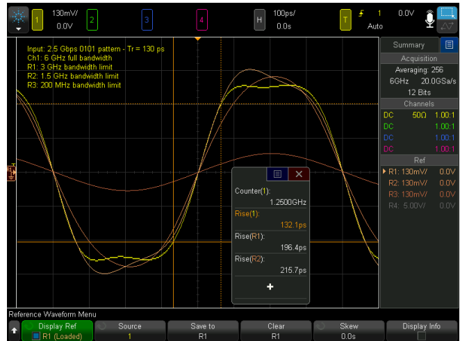
Figure 51. Reference waveforms.
