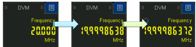
Figure 33. The precise 10-digit counter found the true frequency of a clock to be a little less than 20 MHz.
