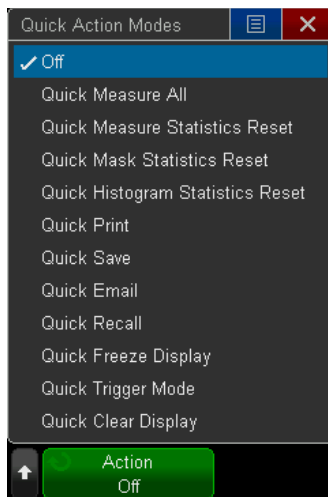
Figure 56. QuickAction menu.
