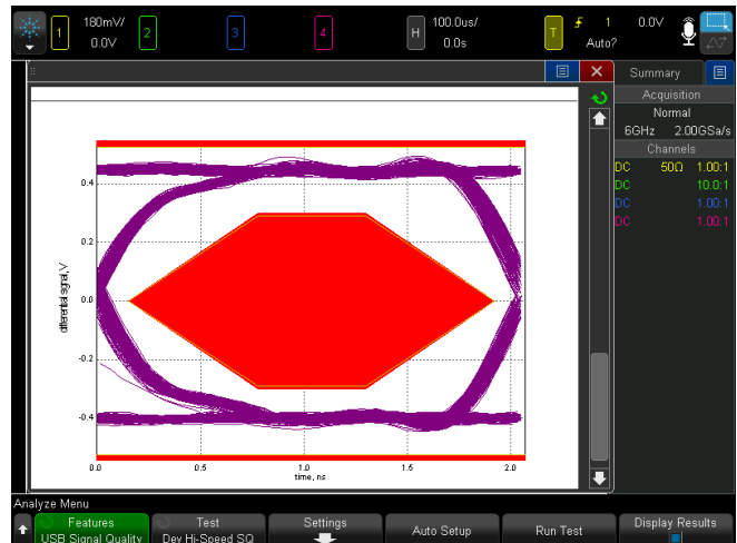
Figure 44. USB 2.0 Hi-speed near-end eye pattern test.
