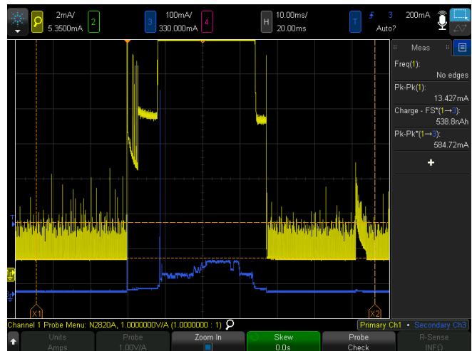
Figure 55. Capturing both zoom out and zoom in view of a cell phone's current consumption inside and outside of its sleep state.
