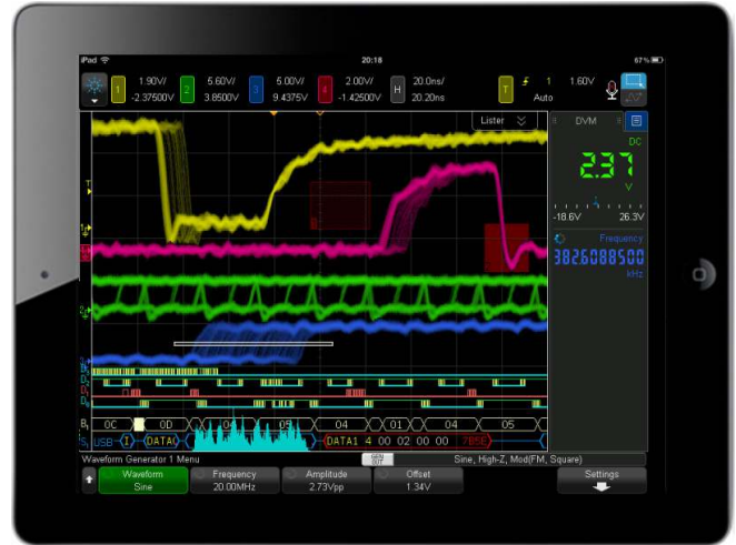
Figure 53. Controlling the 6000 X-Series via tablet device.
