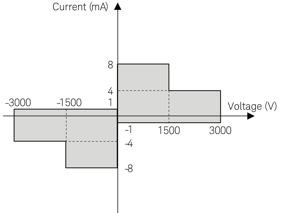
HVSMU measurement and output range
