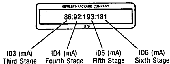
Figure 8-11. A2 Amplifier Bias Currents Label
