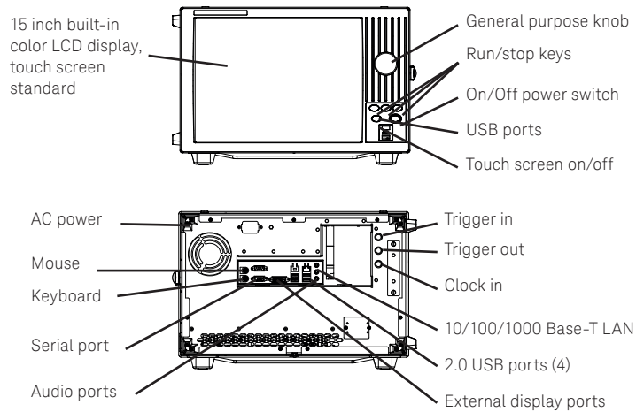
Figure 10. 16850 Series front and back panels.
