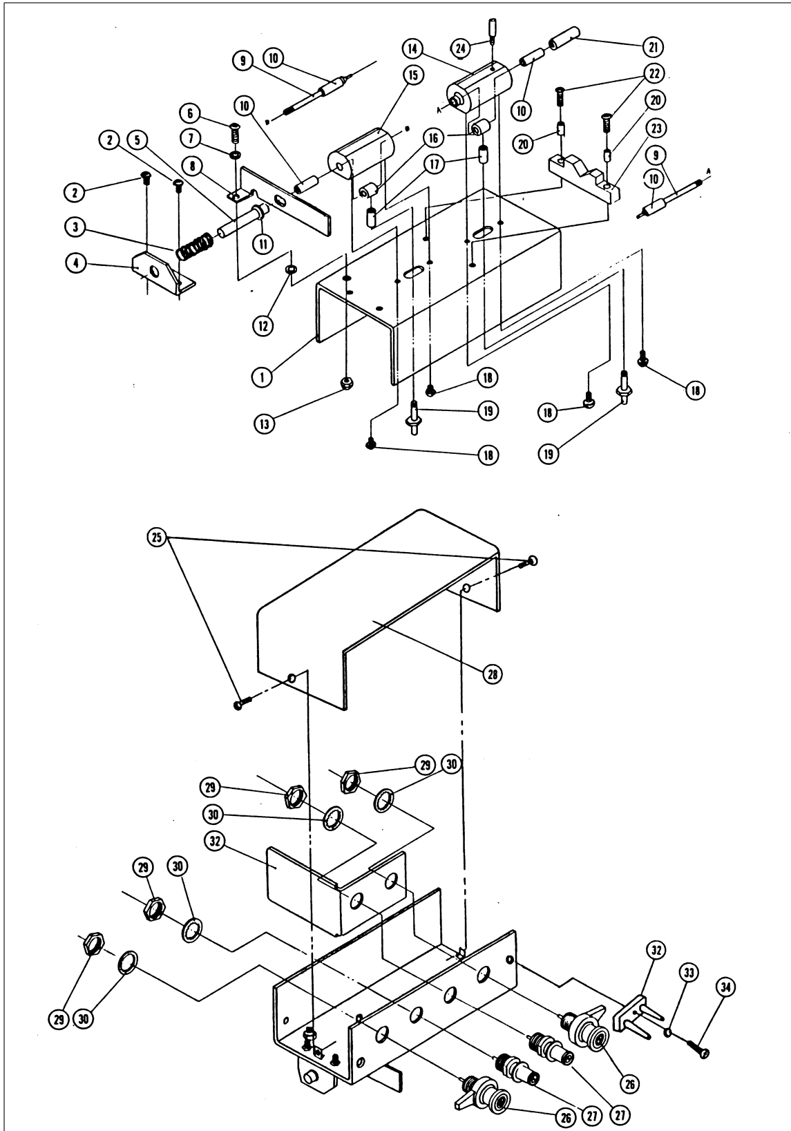
Figure 2-1 Parts Identification
