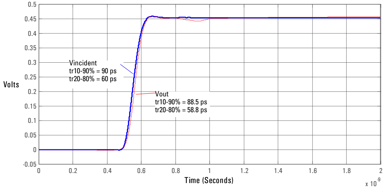
Graph of Vincident and Vout of probe with a 90 ps step.
