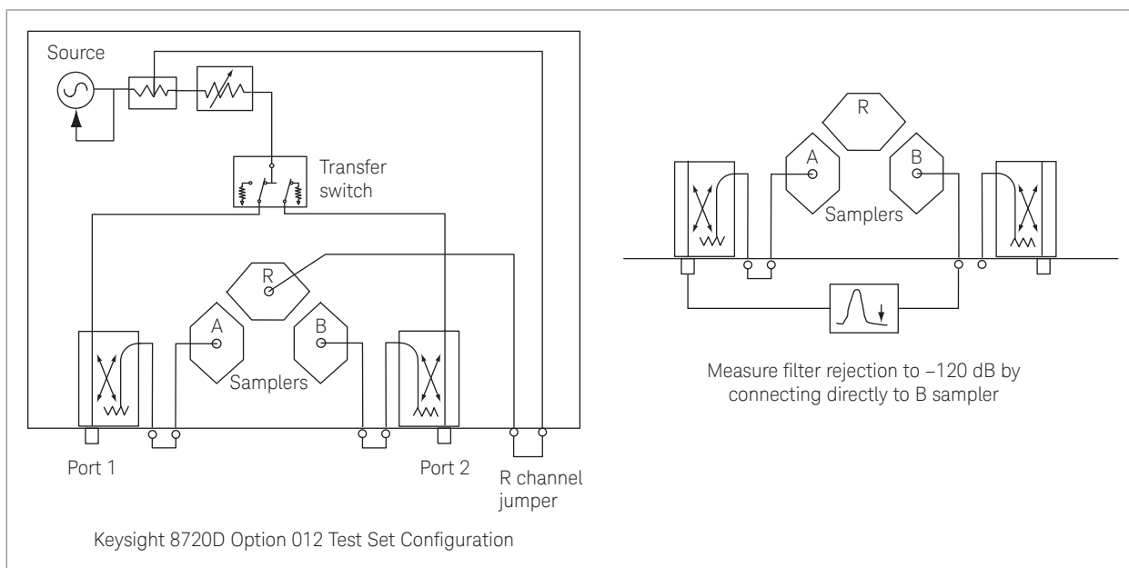
Figure 4. Improving dynamic range with direct sampler access
