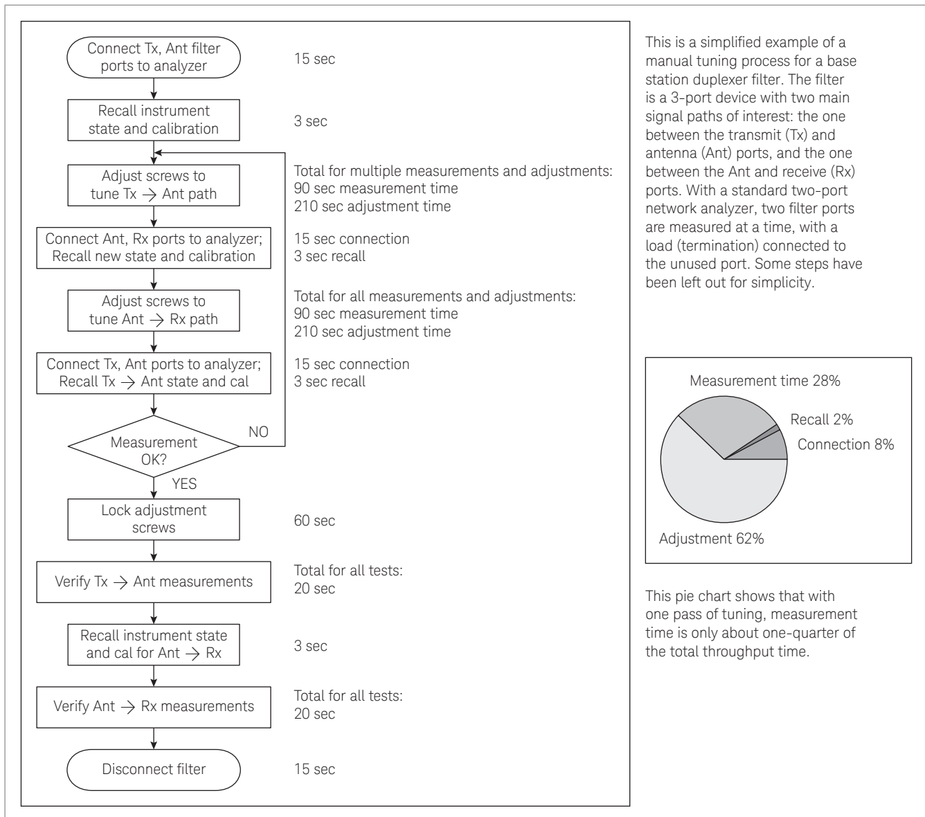
Figure 1. Example manual-tuning process for a base-station filter
