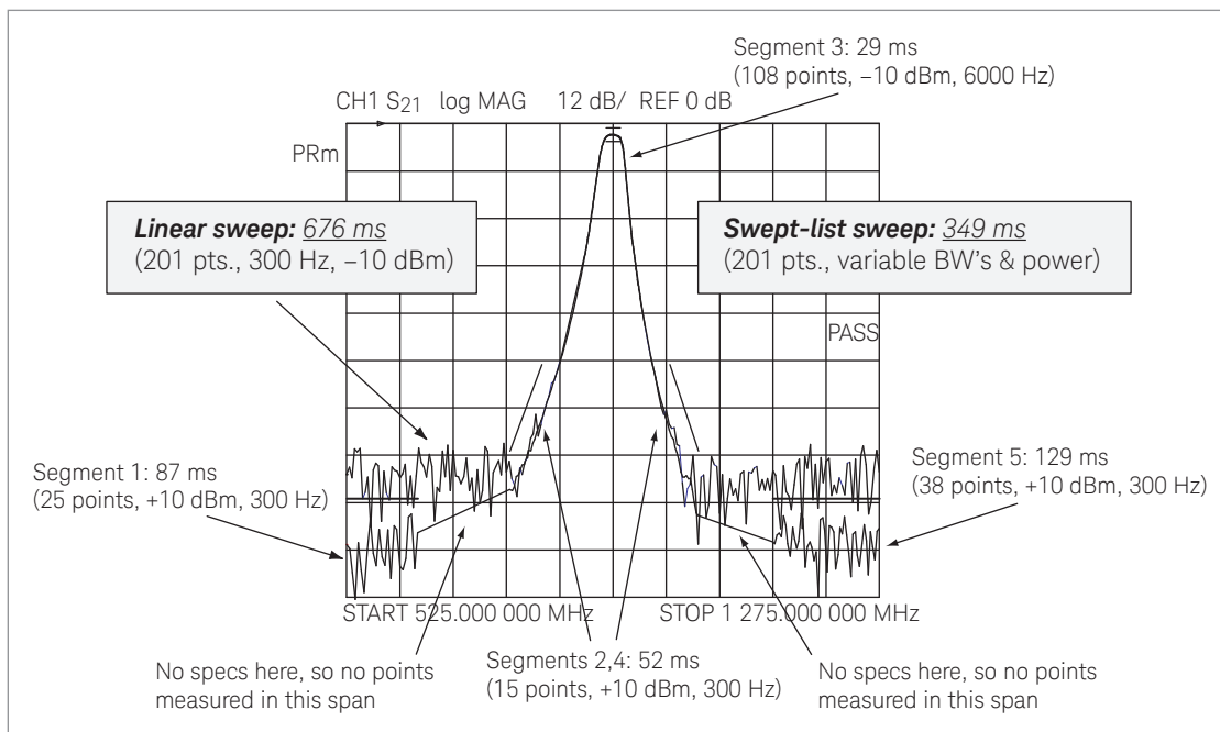
Figure 6. Linear sweep vs. swept list frequency filter measurement
