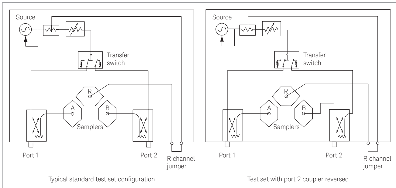
Figure 5. Improving dynamic range with a reversed port-2 coupler
