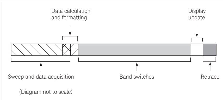
Figure 2. Components of cycle time
