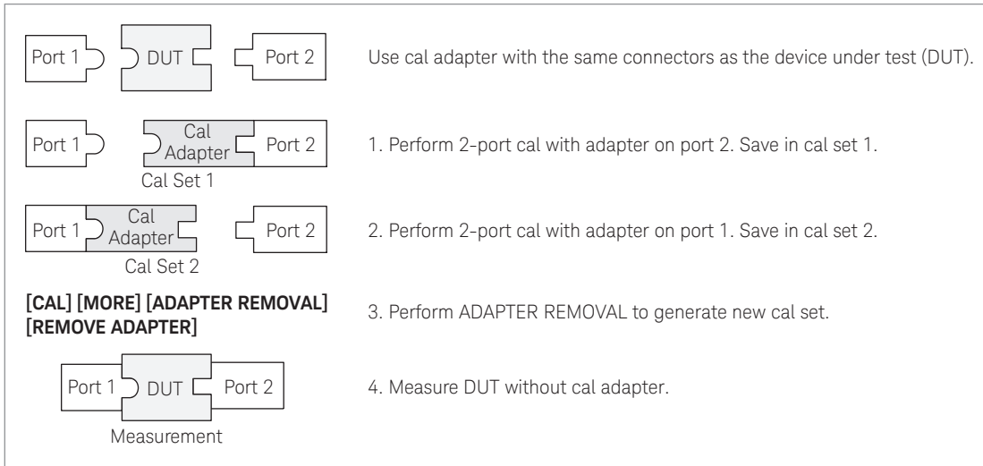
Figure 8. Adapter-removal calibration procedure
