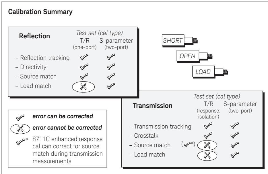
Figure 7. Correctable errors for different test sets and calibration types
