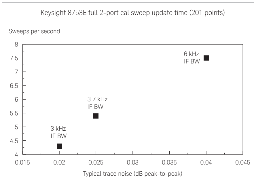
Figure 3. IF bandwidth vs. trace noise and sweep speed
