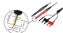
PIN TYPE LEAD L2102 B: 178 mm (7.01 in), L: 1.5 m (4.92 ft)
