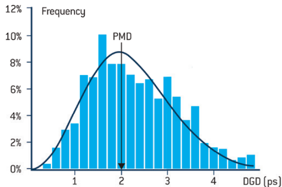
Even with low PMD, high DGD values can occur and lead to PMD compensation failure
