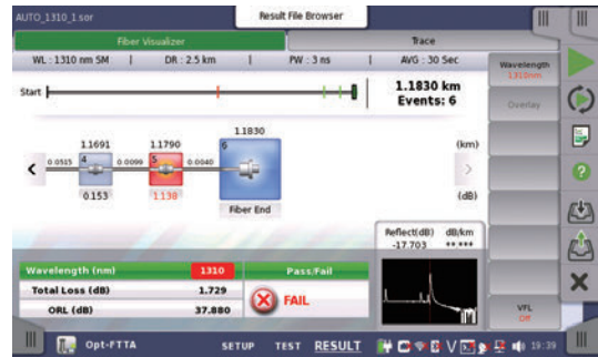
FTTA Measurements
