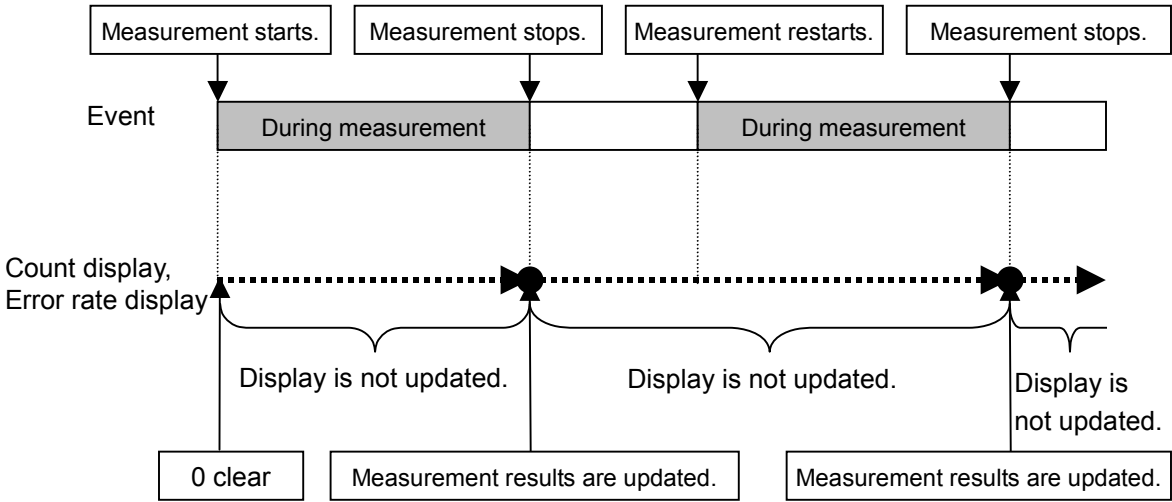
Figure 8.5-8 Measure Mode Continuous
