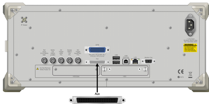
Figure 8.4-1 Input connector
