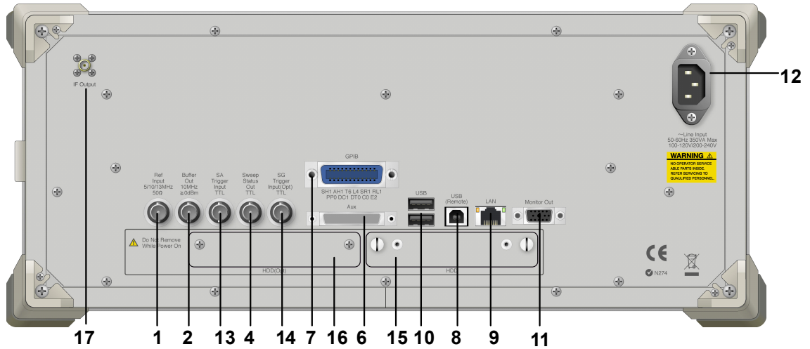
Figure 3.1.1-2 Rear panel
