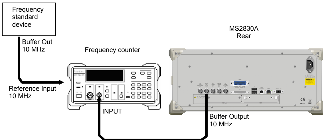
Figure 6.2.1-1 Reference oscillator frequency stability test
