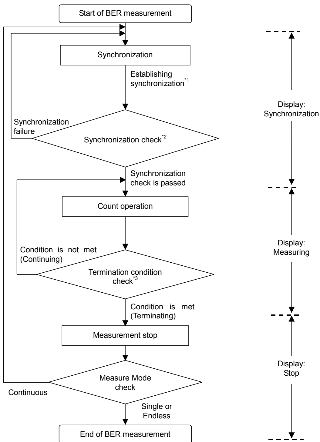
Figure 8.10-1 When Auto Resync is set to Off
