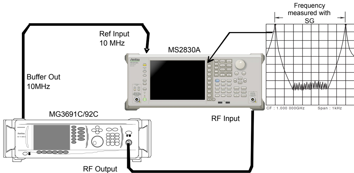
Figure 6.2.3-1 Frequency span display accuracy test
