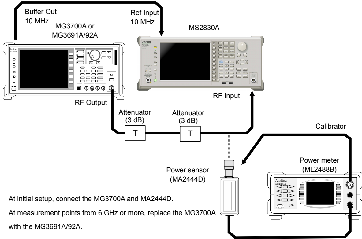
Figure 6.2.5-1 RF frequency characteristics test
