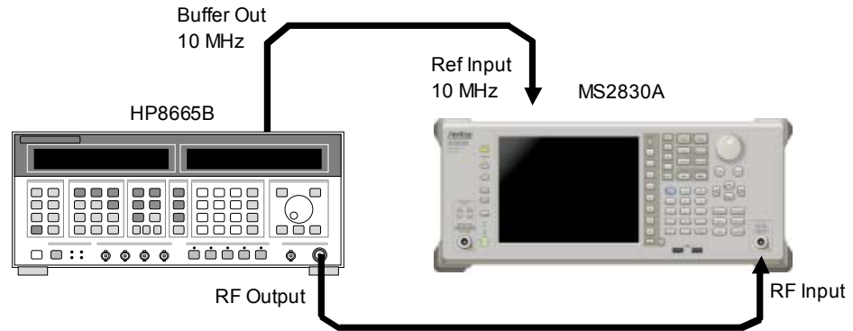
Figure 6.2.4-2 Signal sideband noise level
