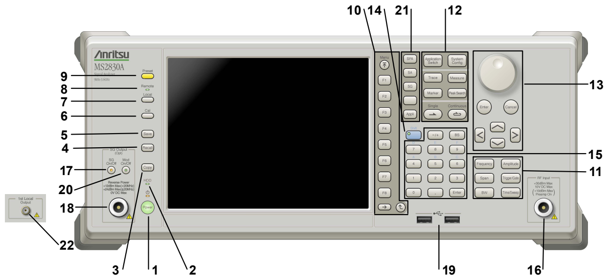
Figure 3.1.1-1 Front Panel
