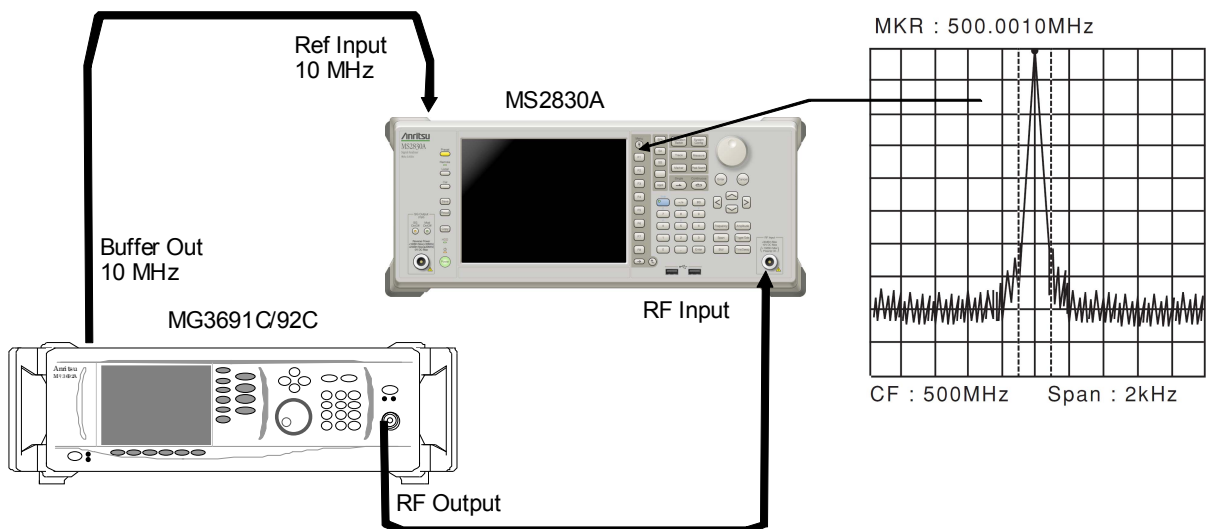
Figure 6.2.2-1 Display frequency accuracy test
