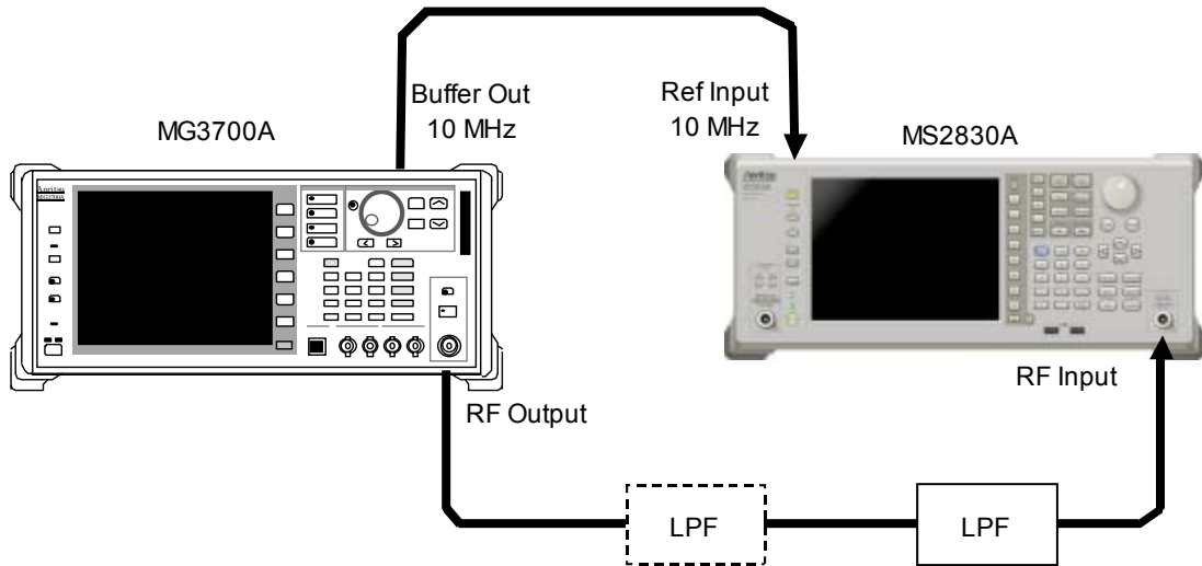
Figure 6.2.7-1 Second harmonic wave distortion test
