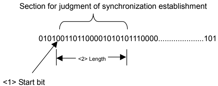
Figure 8.9-6 Setting method for section judged for synchronization establishment
