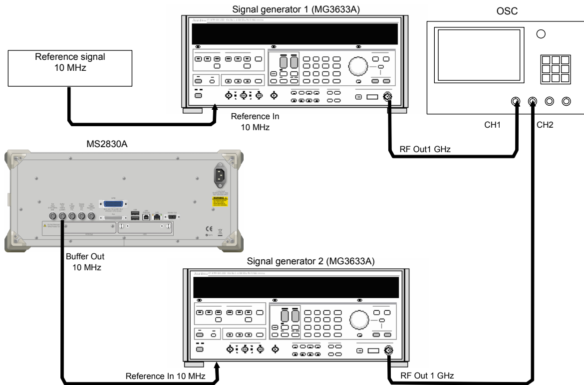
Figure 9.3.3-1 Connections for frequency calibration using oscilloscope
