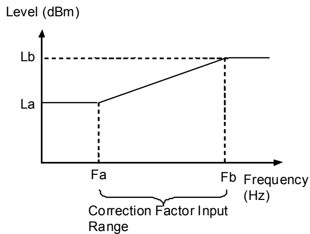
Figure 3.4.10-4 Operation When Correction Factors Are Entered
