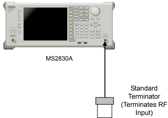
Figure 6.2.6-1 Display average noise level
