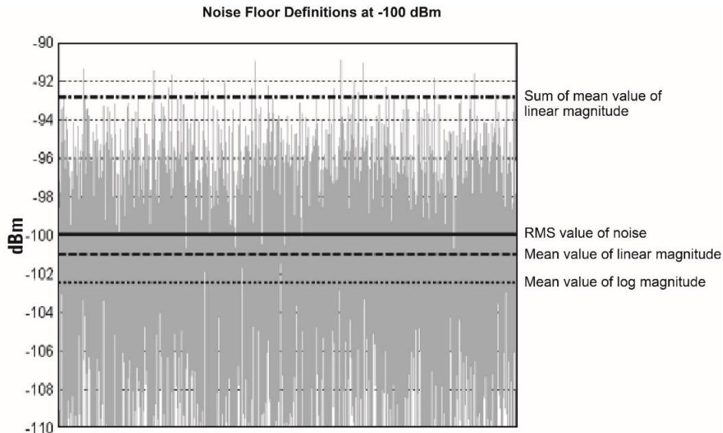
Figure 2. Various noise floor definitions
