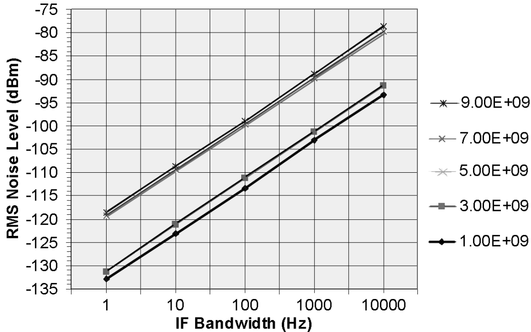
Figure 3. RMS noise floor vs IF BW (n=801 pts)
