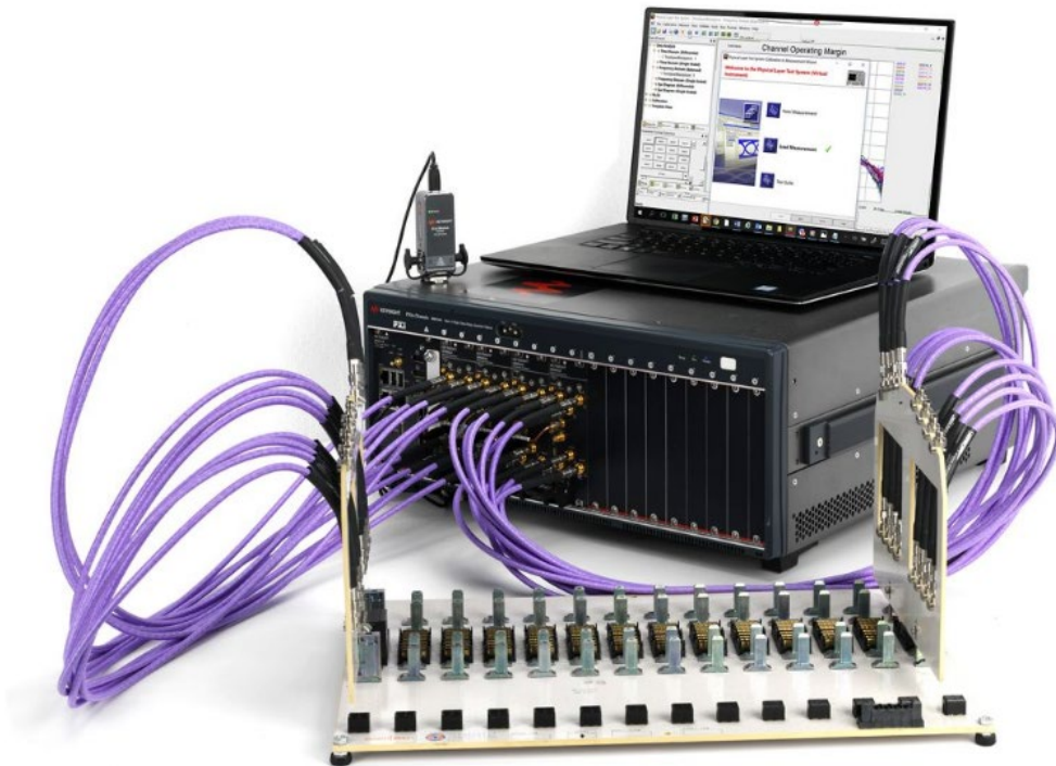
M980xA PXI VNA meets the most demanding multiport challenges with a true multiport architecture.
